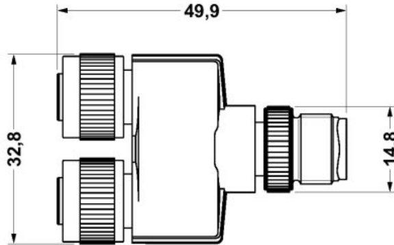
Dimensioned drawing
