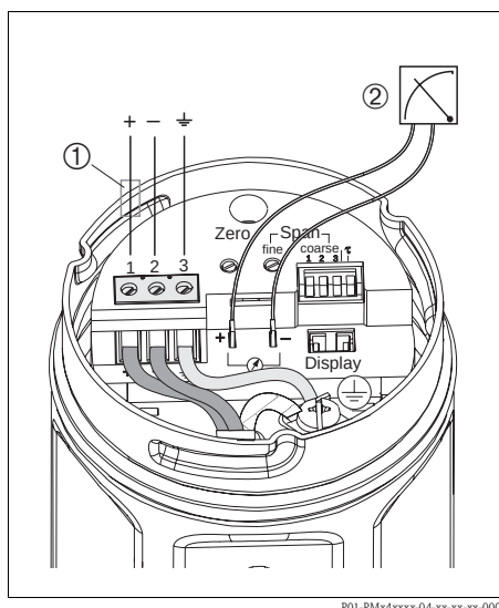
Analog electronic insert
