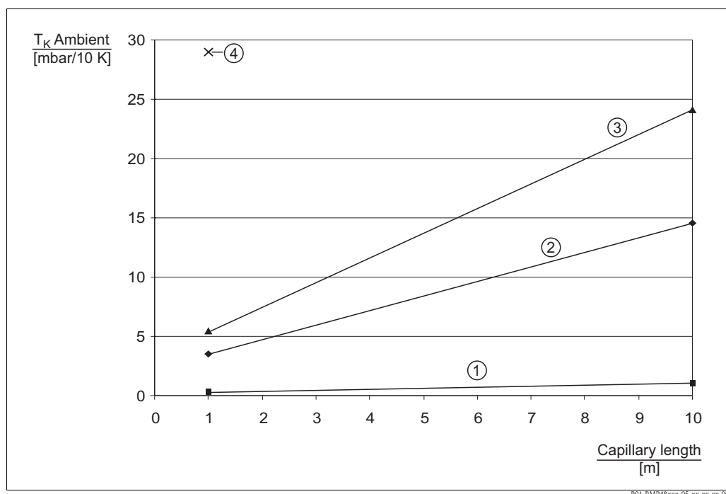
Diagram T_K \text{ Ambient} as a function of the capillary length for PMP48
