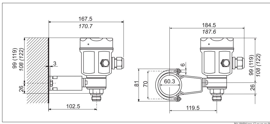
Wall and pipe-mounting PMP41
