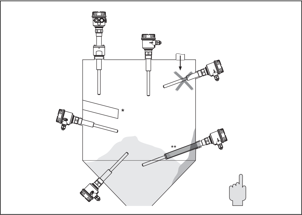
Horizontal installation/vertical installation * With protective cover (to be provided by customer) ** With protecting tube (to be provided by customer)
