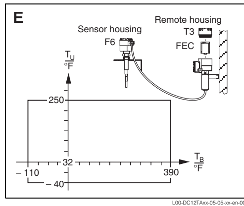
Basic probe and electronic insert in remote housing
