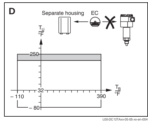
Probe with temperature spacer and electronic insert in separate housing
