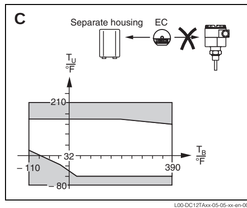
Electronic insert in separate housing
