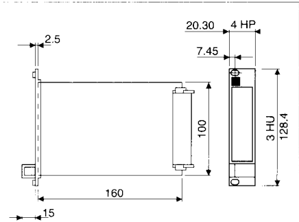
Dimensions (mm), 1" = 25.4 mm
