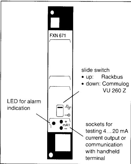
FXN 671 power supply unit
