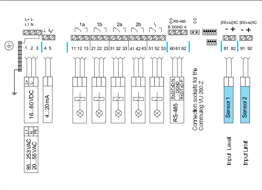
Terminal strip of the FMC 661—the electrically isolated circuits are indicated by the blue lines
