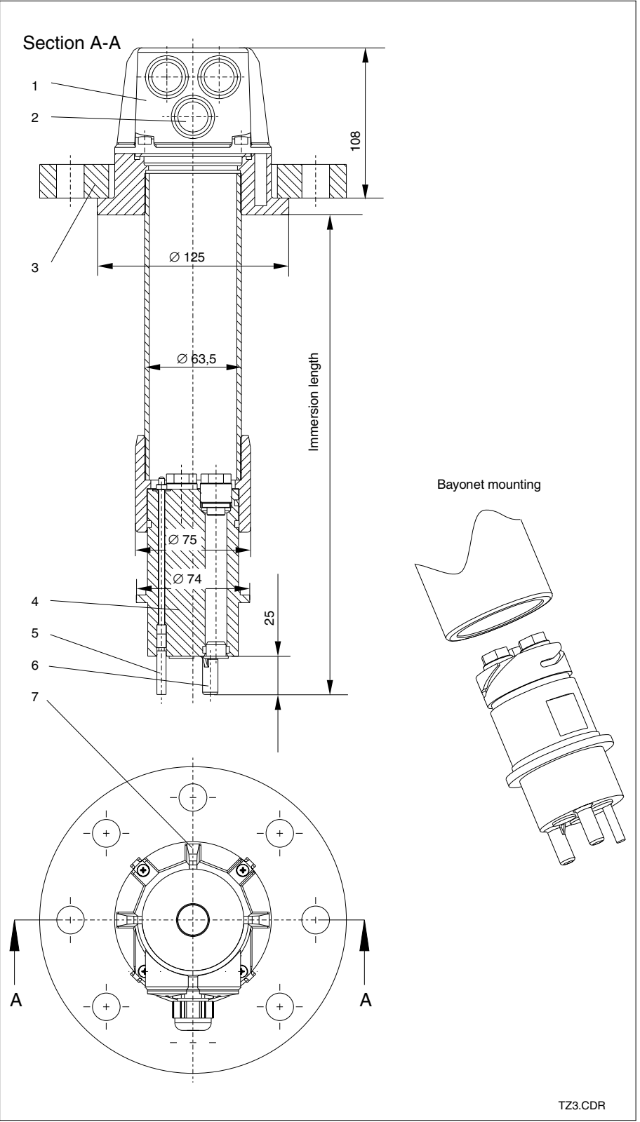
Dimensions of the PVDF assembly DipFit P CPA 140 1 Assembly head 2 Cable gland Pg 13.5 3 Loose flange 4 Electrode holder 6 Shock-protection studs 7 Goretex® filter
