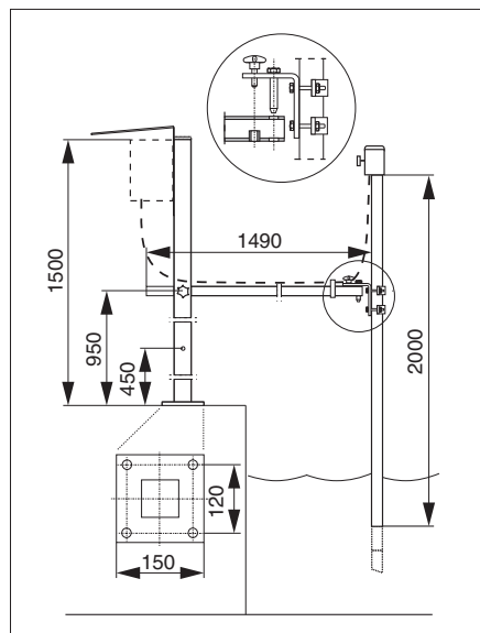
Assembly holder CYH 101 with weather protection cover CYY 101 for field transmitter
