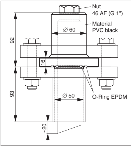
left: CUA 120-B adapter with welding neck DN 50 / ANSI 2" (accessory) and lap joint flange DN 50 / ANSI 2" (to be provided by customer)
