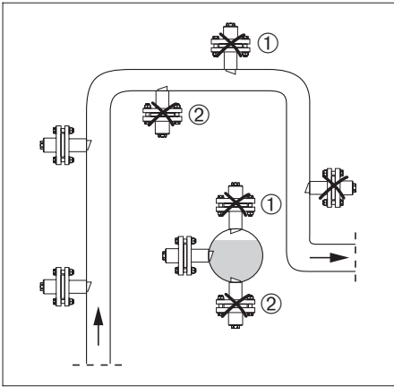
Orientation and positions of CUS 41 with CUA 120-A/-B adapter or CUA 461 retractable assembly
