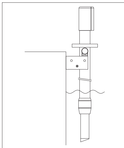
TurbiMax W CUS 41 sensor installed in CYA 611 assembly with pendulum frame
